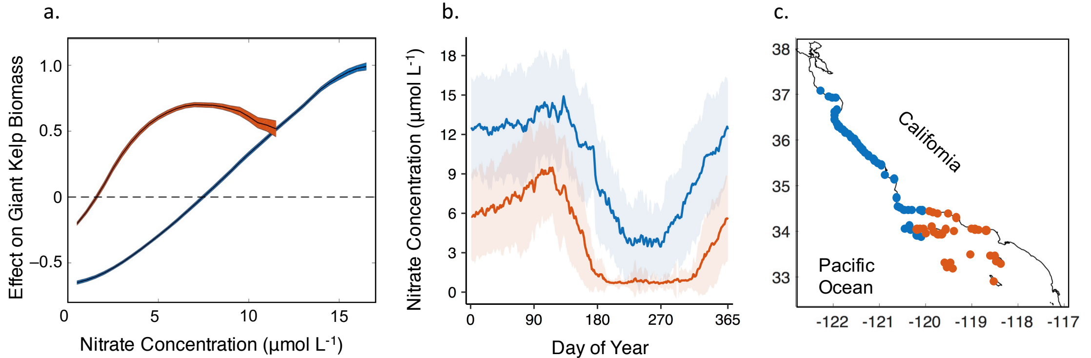
Figure S1. a.) Mean nonlinear response curves showing the relationship between giant kelp canopy biomass and seawater nitrate concentration for the two populations, shaded areas show standard error. b.) Mean annual seawater nitrate time series for the two populations, shaded areas show 95% confidence intervals. c.) Map of the coastline of California showing the geographic clustering of each coastline segment's response curve to nitrate concentration using a kmeans clustering analysis.
