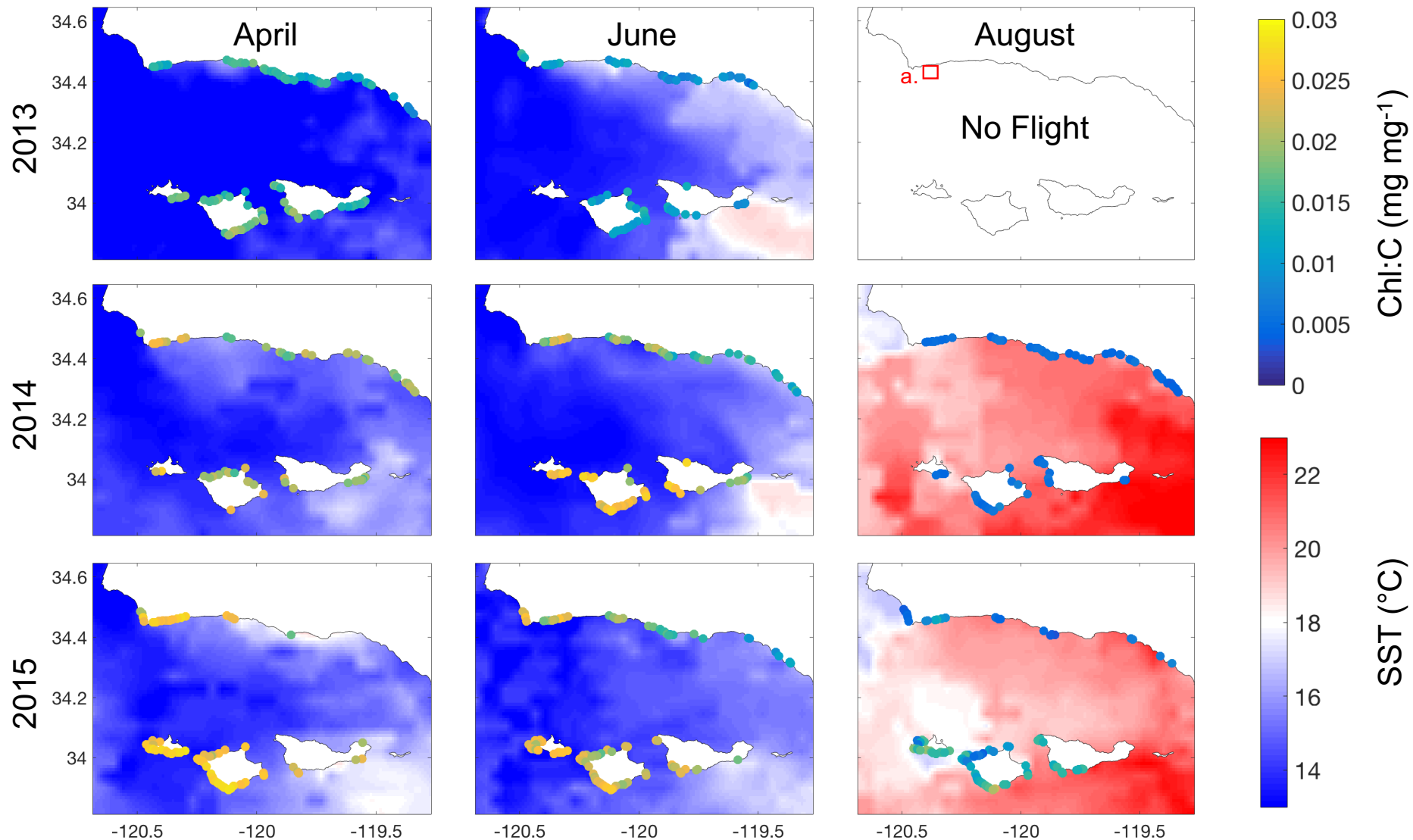
Figure S2. Maps showing the mean canopy chlorophyll a to carbon ratio (Chl:C) for each 1 km coastline segment estimated from Airborne Visible/Infrared Imaging Spectrometer (AVIRIS) imagery. The background of each map shows the mean sea surface temperature (SST) for the 16-day period prior to the AVIRIS image date for the Santa Barbara Channel at 4 km resolution from the MODIS Aqua sensor. Red box (a.) shows the location of Figure 2 in the Statement of Research.
