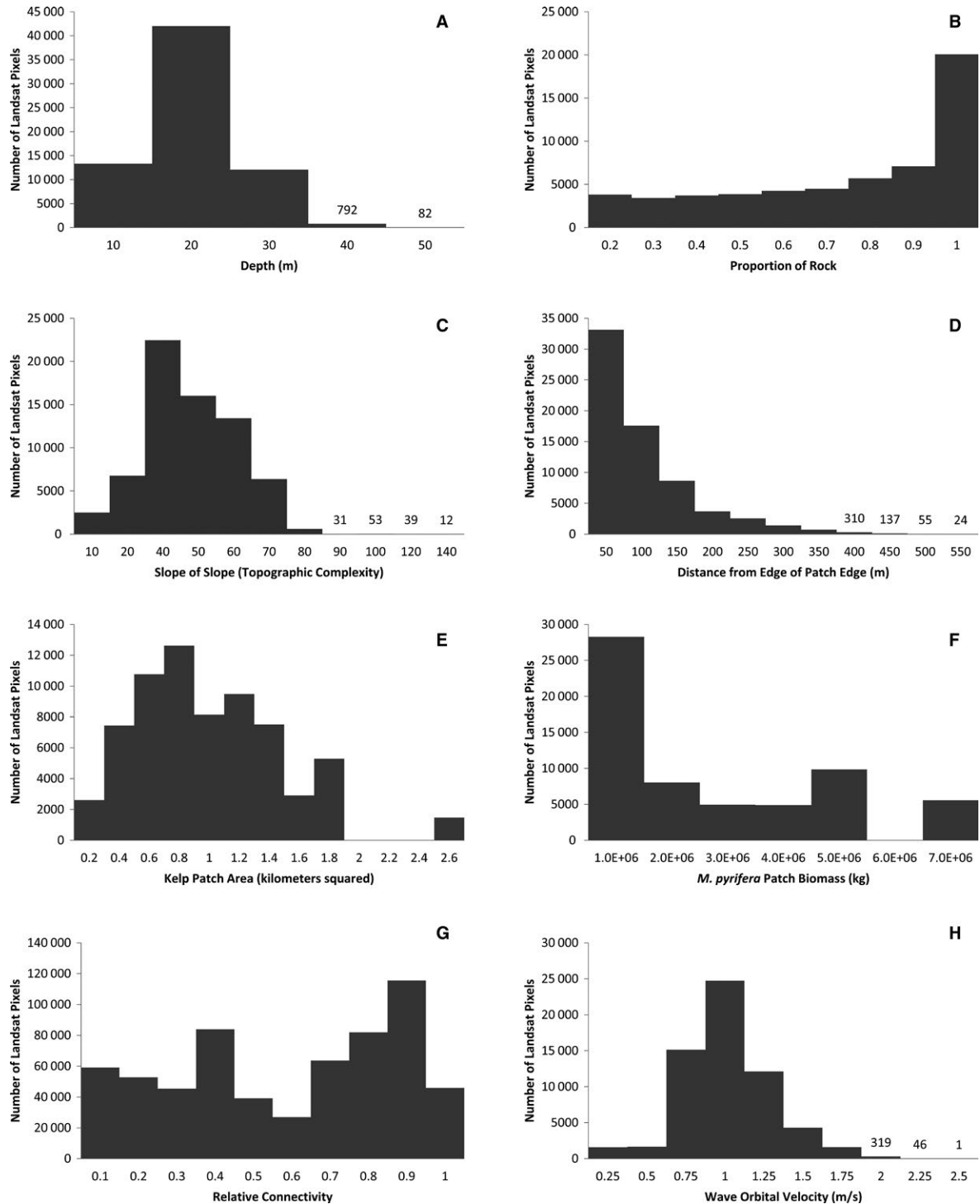
Fig. 4. Frequency distributions of the occurrence of Macrocyctis pyrifera in relation to (A) variation in depth, (B) proportion of rock, (C) slope of slope or topographic complexity, (D) distance from edge of kelp patch, (E) kelp patch area, (F) total biomass within a kelp patch, (G) the relative connectivity of the patch, and (H) the wave orbital velocity. Vertical axes are the number of Landsat pixels where kelp is present within each of the categories of geomorphic structure.
