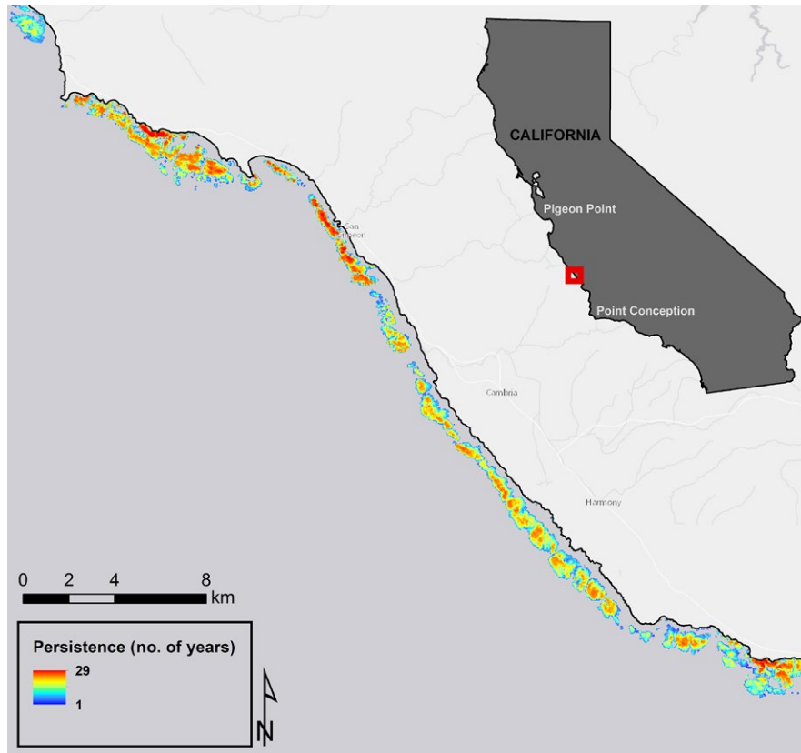
Fig. 2. The persistence of Macrocyctis pyrifera along a small portion of the central coast of California. The warmer colors represent higher persistence (greater number of years when M. pyrifera is present in a certain location) compared to the cooler colors, which represent areas where M. pyrifera is less persistent. Persistence is measured at 30-m resolution (the resolution of the Landsat data). Service Layer Credits for ESRI grayscale background image: Copyright 2013 Esri, DeLorme, NAVTEQ.
