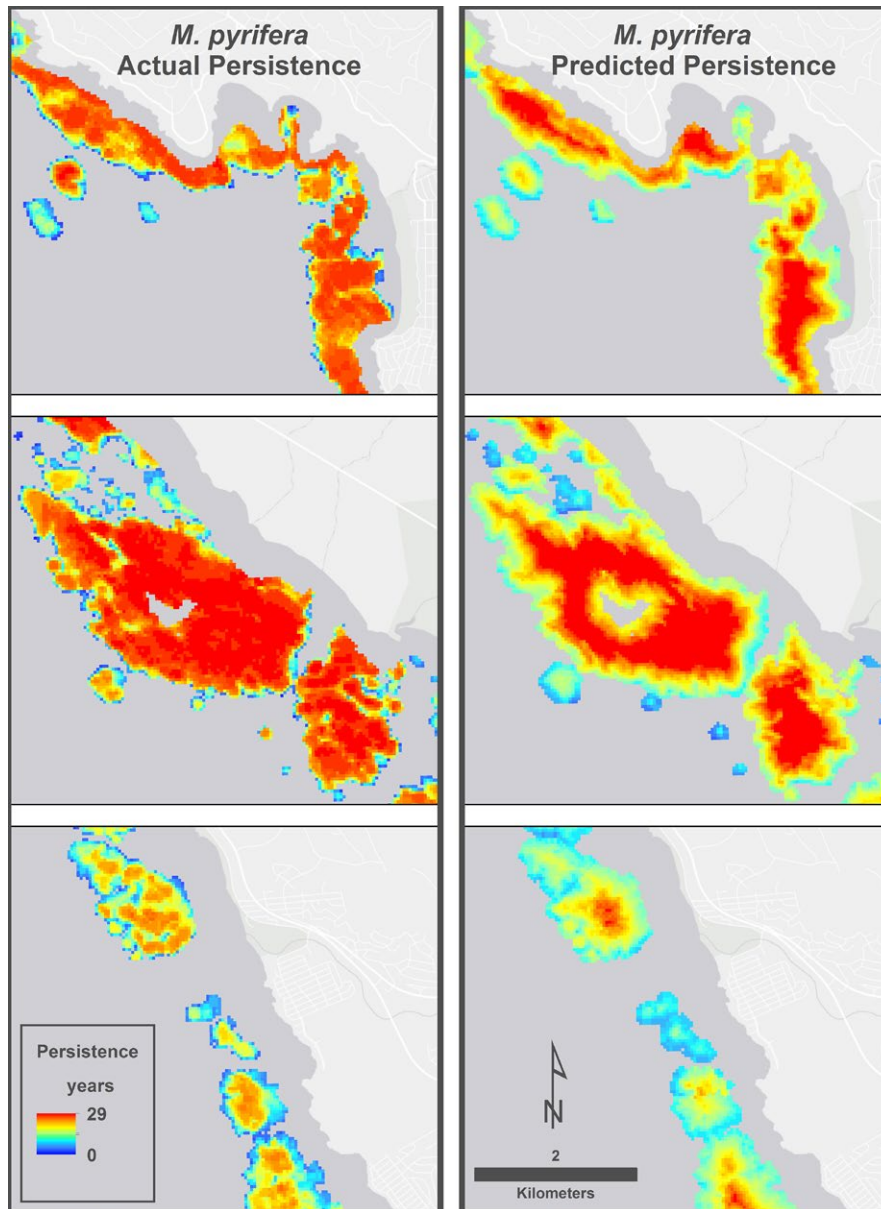
Fig. 6. Comparison of actual Macrocyctis pyrifera persistence (left panel) and persistence predicted from the GLMMs (right panel) in three locations along California's central coast. Persistence is given in number of years with the warmer colors (reds, oranges) representing areas of higher persistence and cooler colors (blues) representing areas of lower persistence. Both the actual and predicted persistence maps are at 30-m resolution. Service Layer Credits for ESRI grayscale background image: Copyright 2013 Esri, DeLorme, NAVTEQ.
