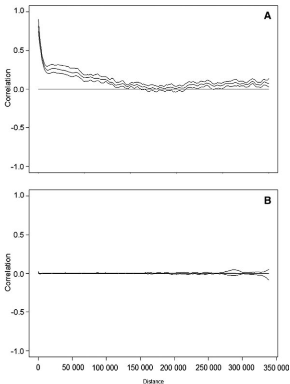
Fig. 5. Spline correlograms with 95% pointwise bootstrap confidence intervals showing the comparison of (A) the spatial autocorrelation of the residuals of a generalized linear model (GLM), which does not take into account spatial autocorrelation, and (B) the spatial autocorrelation of the residuals from the generalized linear mixed model (GLMM). The correlation of the residuals at close distances (measured in meters) in the GLM were significantly correlated, whereas there is almost no spatial autocorrelation at any distance class in the GLMM.
