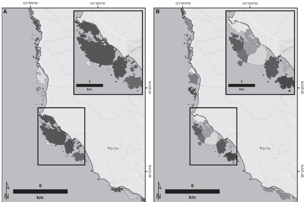
Fig. 3. Examples of (A) the contiguous patches used to calculate the patch variables and (B) the subpatches used to calculate the connectivity between the subpopulations. The different levels of gray in both maps represent different patches and the inset maps show a close-up view of one area of patches to highlight the variation in the different methods for defining patches within the central coast of California. Service Layer Credits for ESRI grayscale background image: Copyright 2013 Esri, DeLorme, NAVTEQ.
